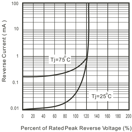
Fig. 1 - Reverse Characteristics
